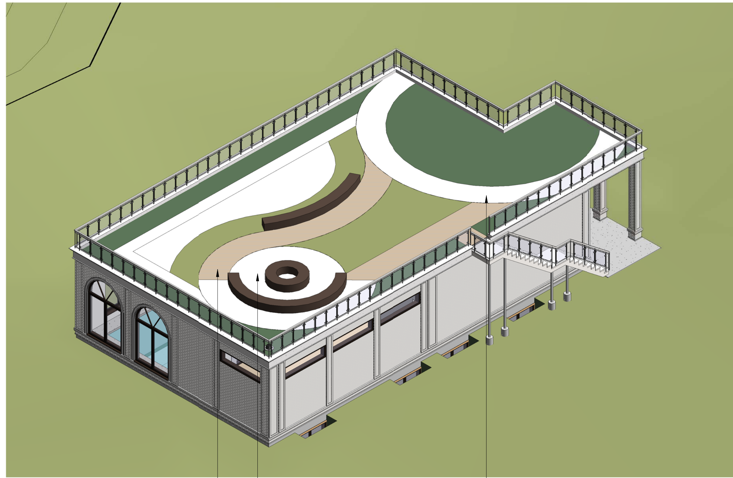
① 3D VIEW - ROOF 1
